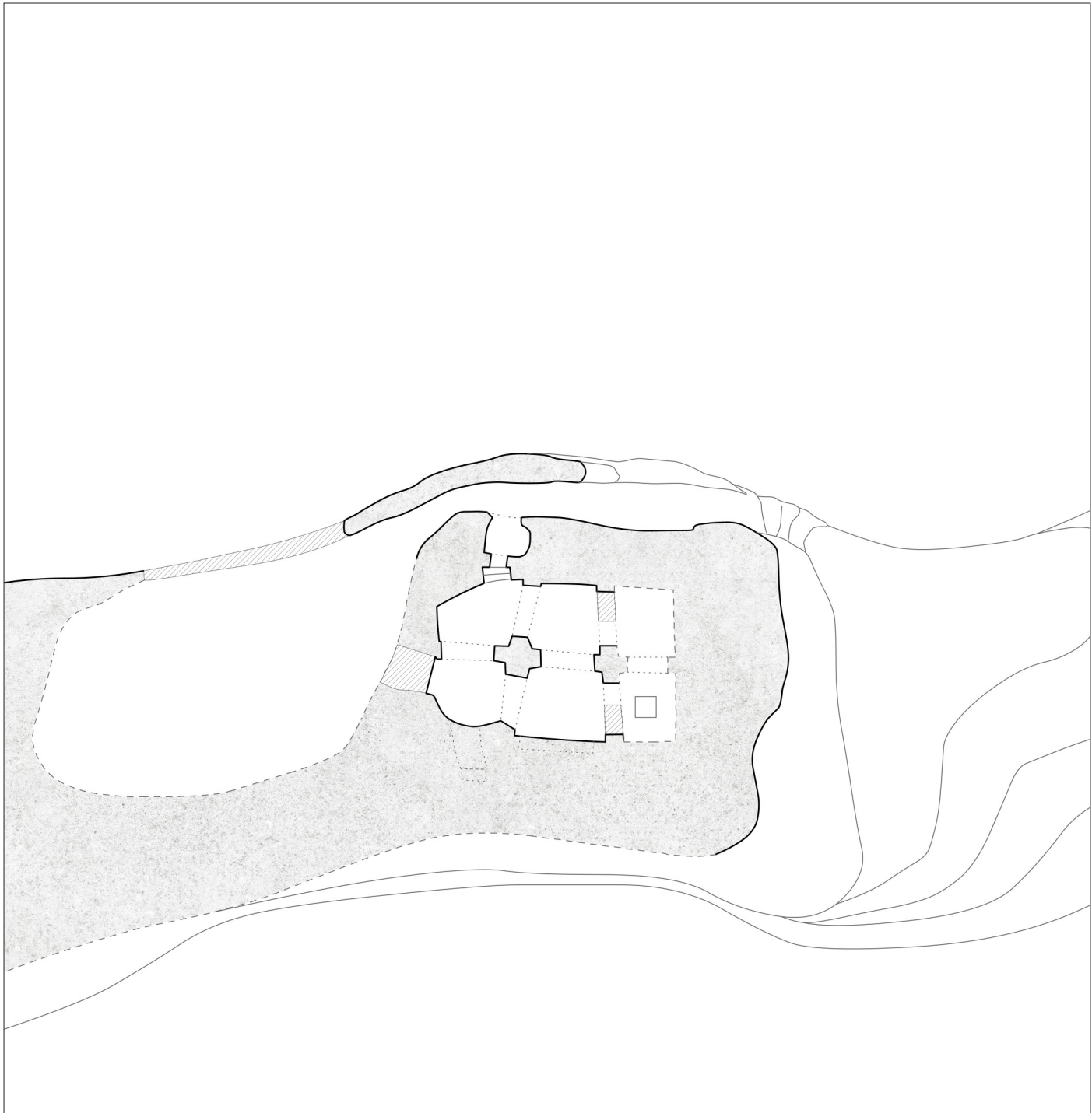
Arbatu Ensesa Kemer Ground Floor Plan (2016)
